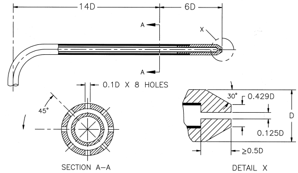
c. Alternate Pitot-Static Tube with Blunt Head
